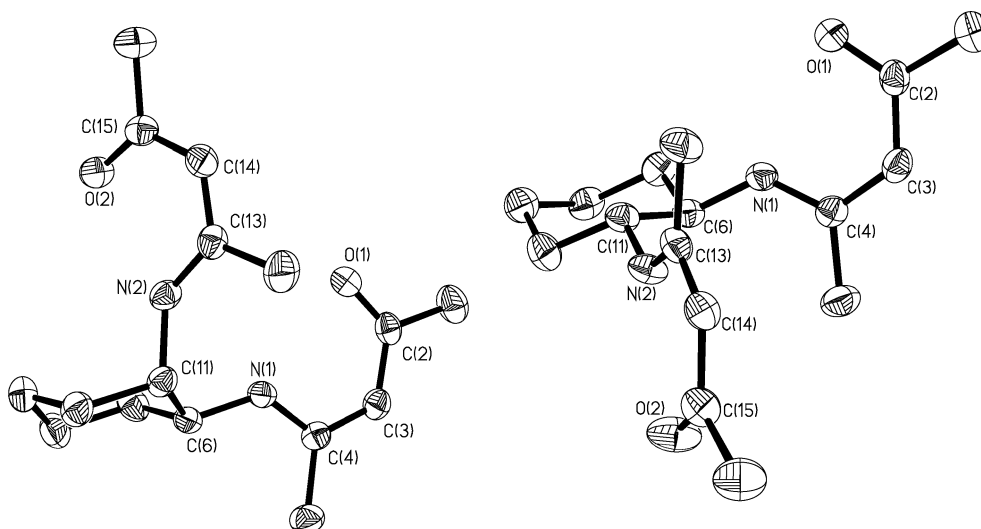
Figure 2. The comparison of the molecular structures of cis - and trans -1, in which thermal ellipsoids were drawn at 30% probability and all hydrogen atoms were omitted for clarity.
