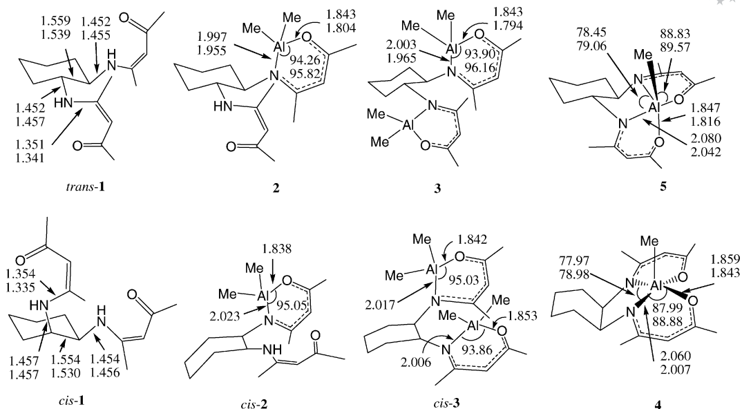
Figure 1. Structures and geometrical parameters obtained at the B3LYP/6-31G* level. The parameters obtained by X-ray diffraction data are shown in the second entries.
